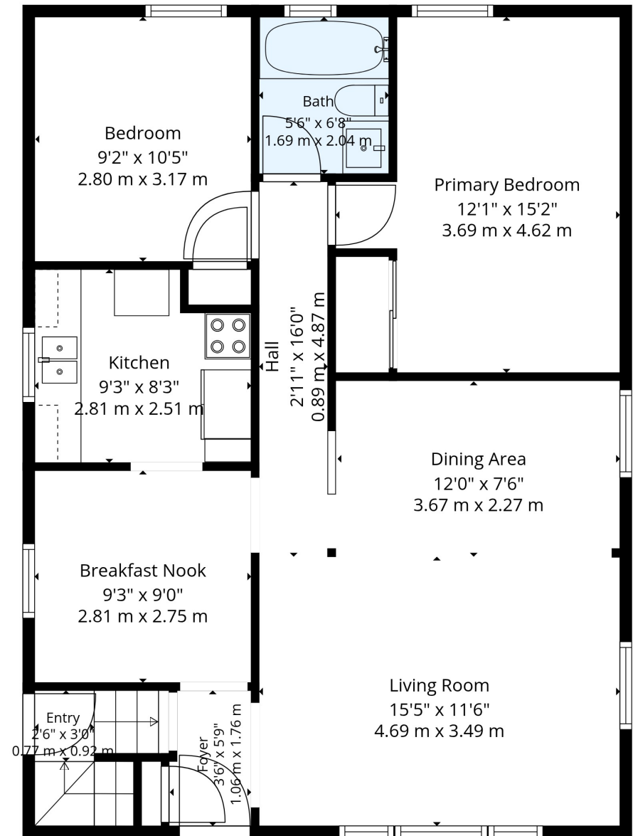
2nd Floor
