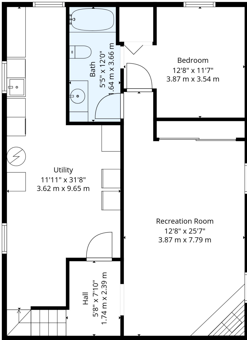
1st Floor
