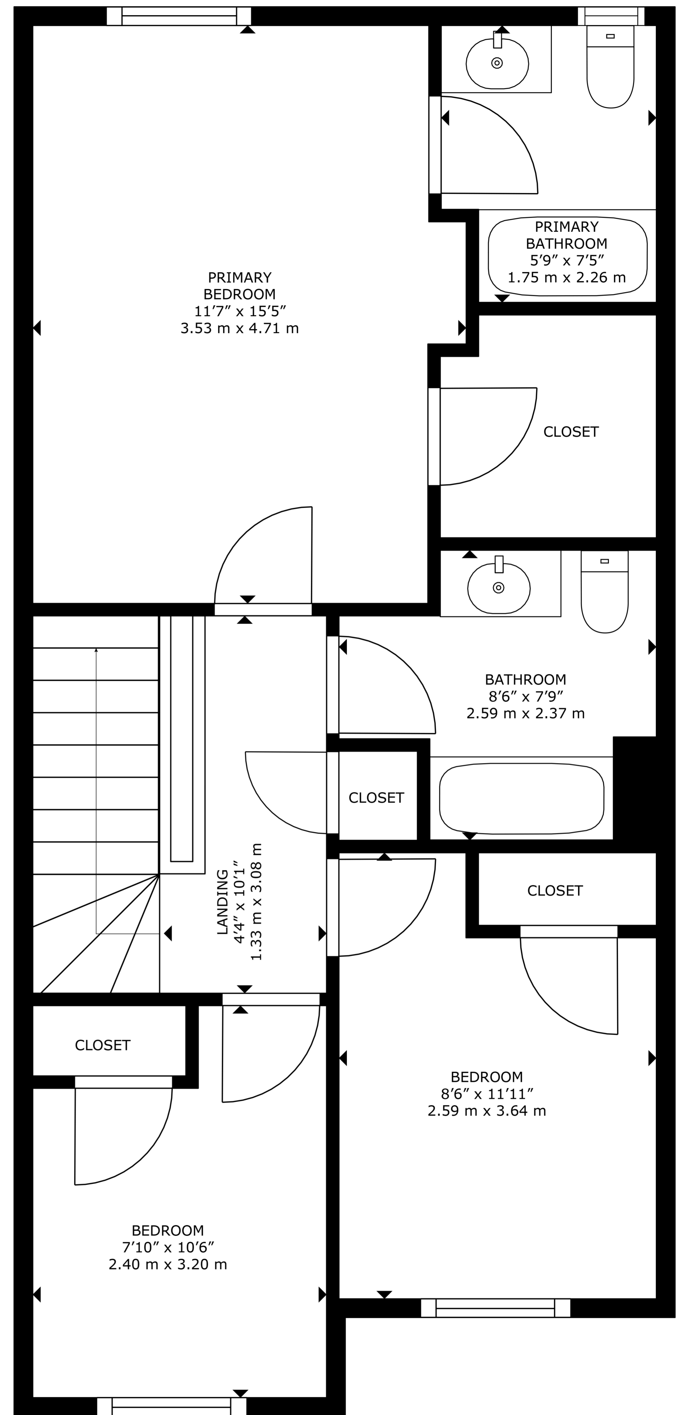
FLOOR 3
