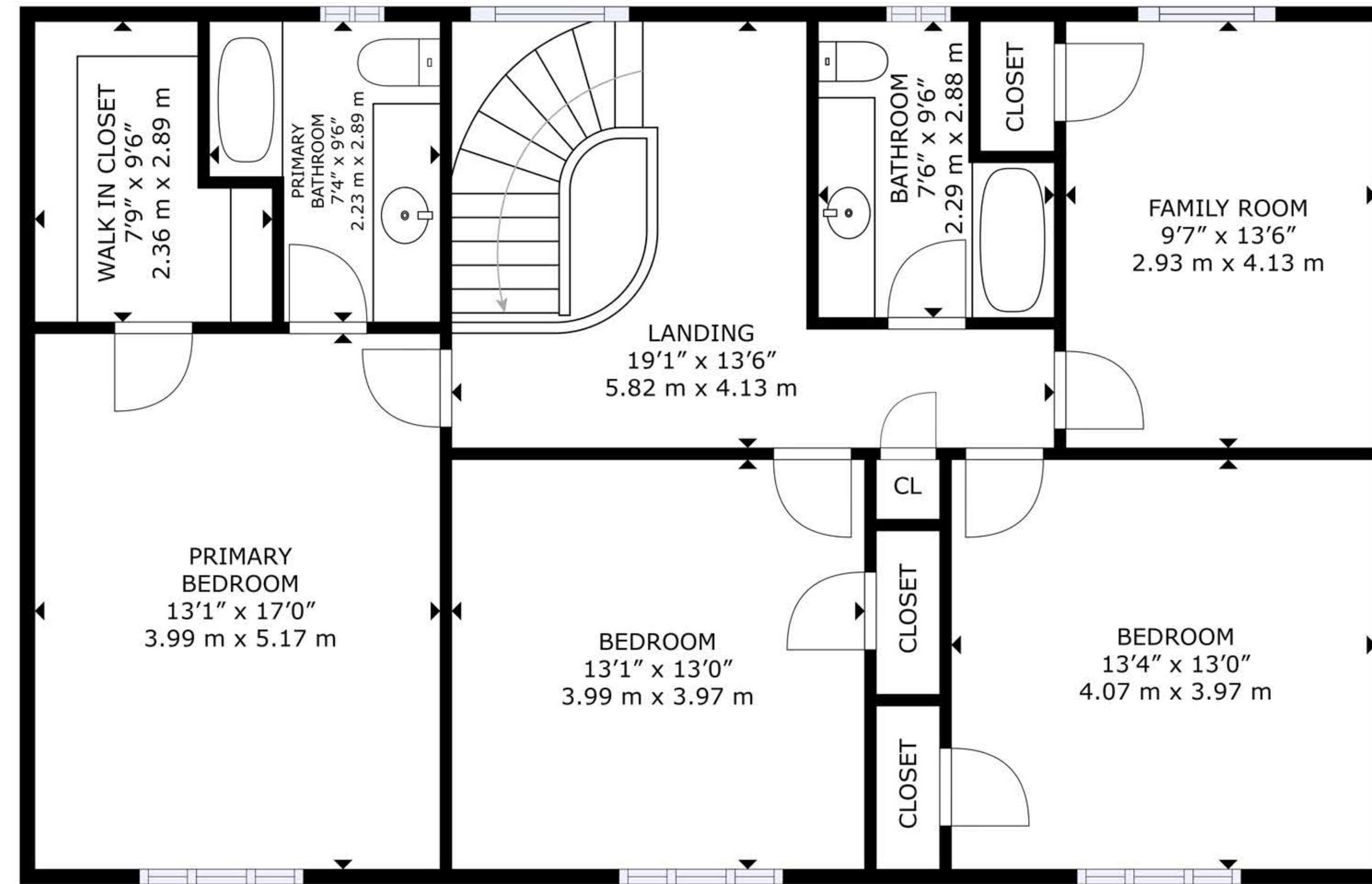
FLOOR 2
