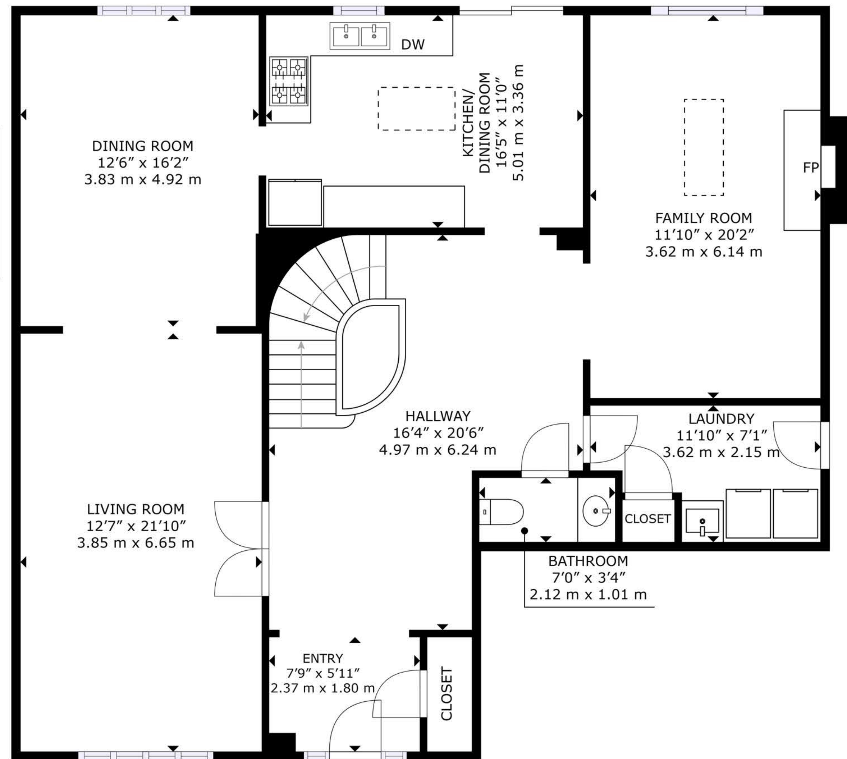
FLOOR 1
