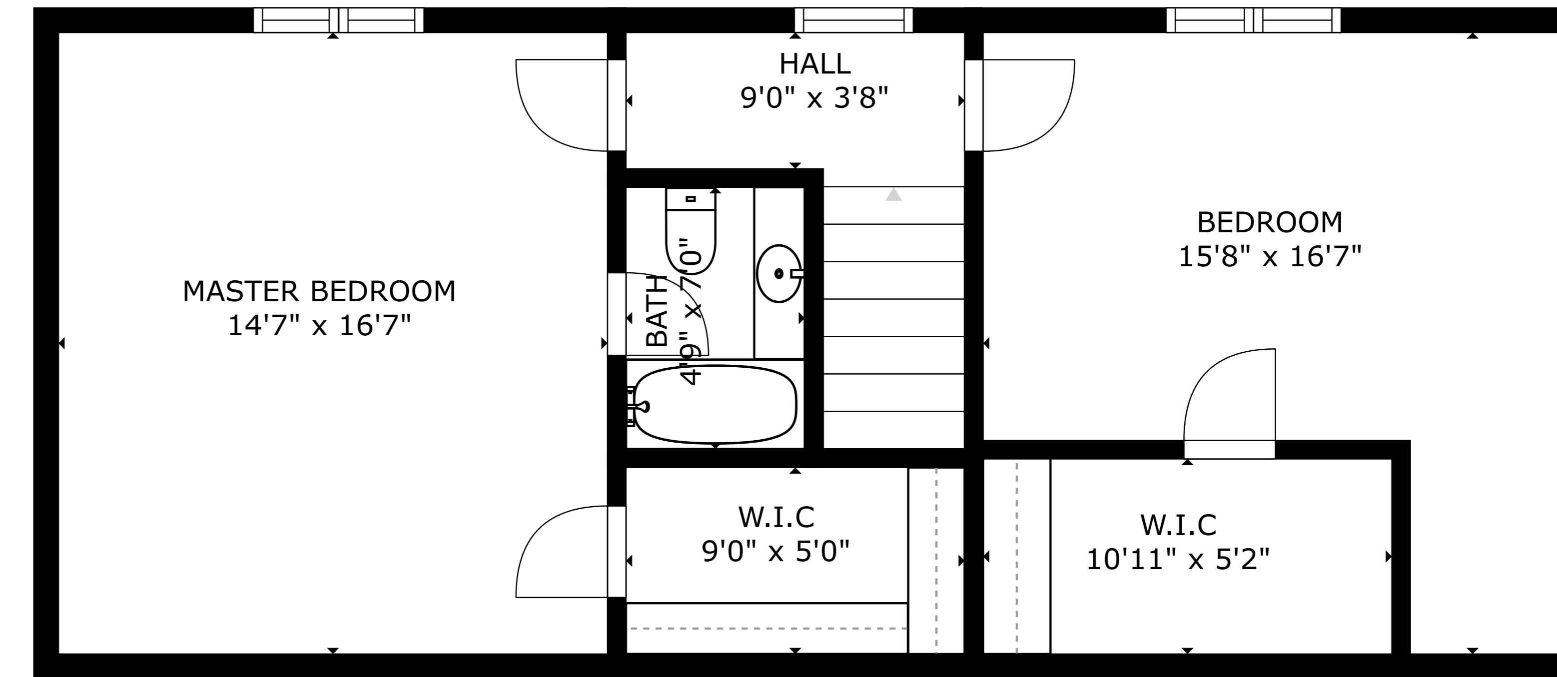
SECOND FLOOR
