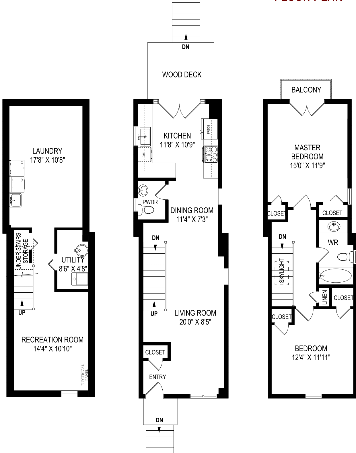
LOWER LEVEL FLOOR PLAN 562 SQUARE FEET
