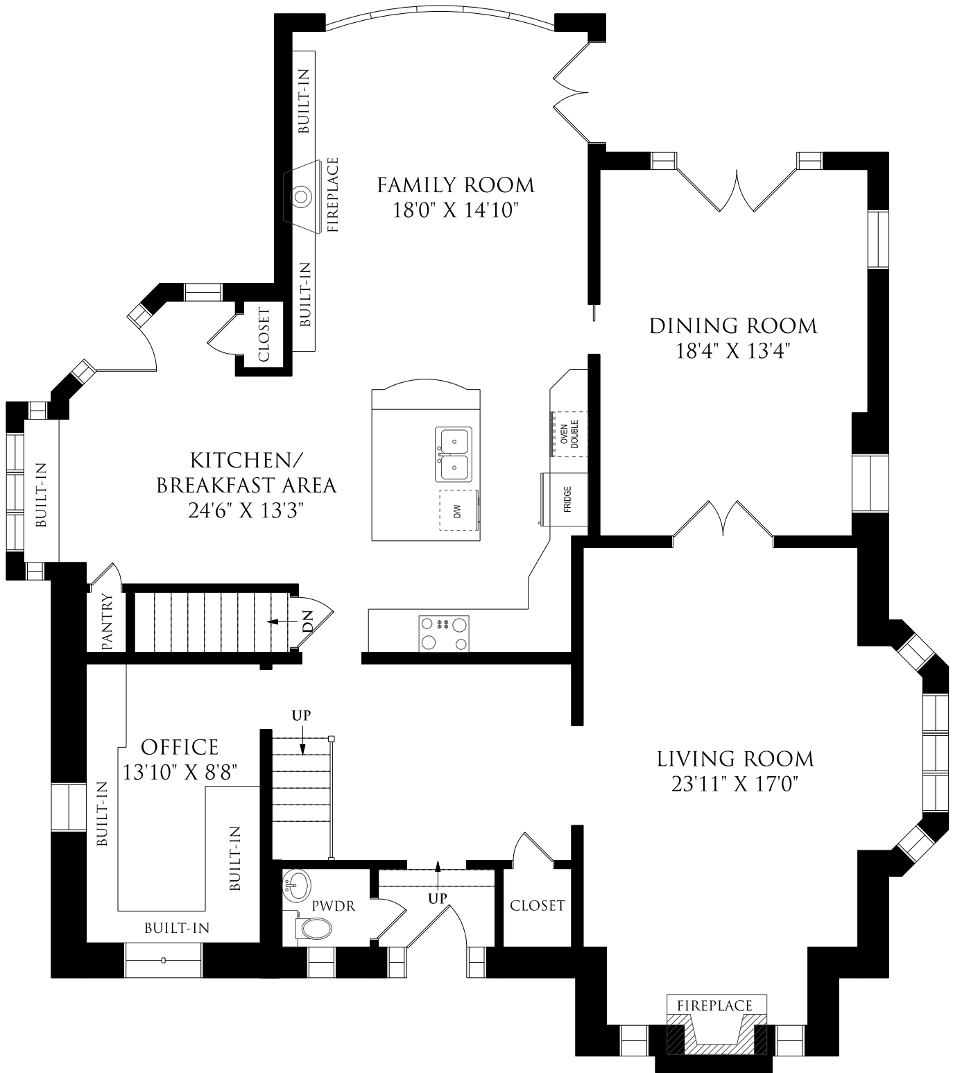
MAIN FLOOR 1869 SQUARE FEET
